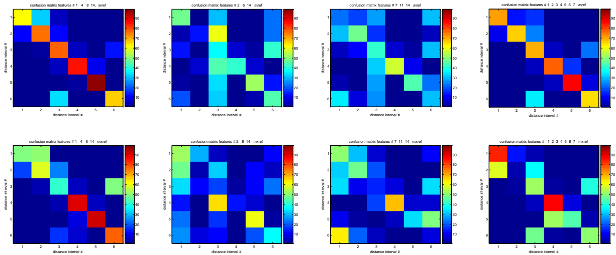
Figure 19: Confusion matrices (%) between 6 distance intervals for four sets of features with feature references obtained by averaging (top row) and by maxing (bottom row).
