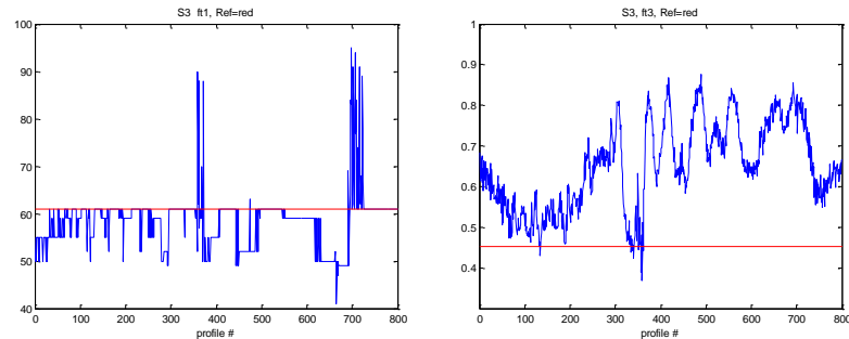
Figure 21: Values of features 1 & 3 (ship S3) as a function of distance (red line = reference from table 2).
