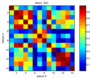
Figure 7: cross correlation coefficients \text{abs}(\rho) \in [0 \ 1] between all 14 features.
