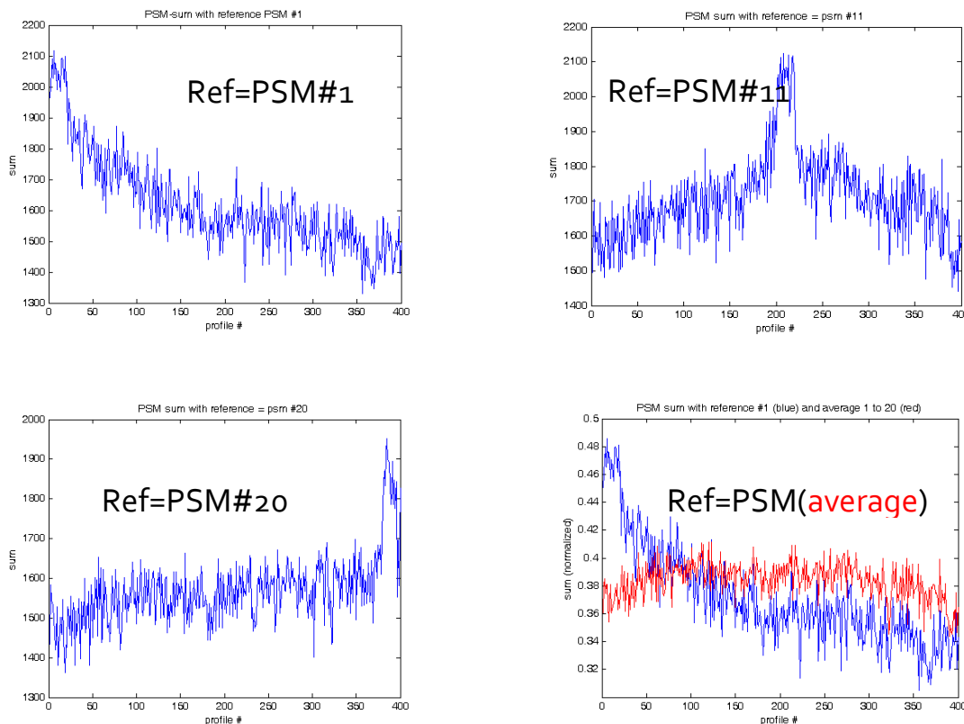
Figure 16: Three examples of the FoM (top and lower left). At the lower right the normalized FoM is shown in a comparison between PSM #1 (blue) and the average PSM (red).
