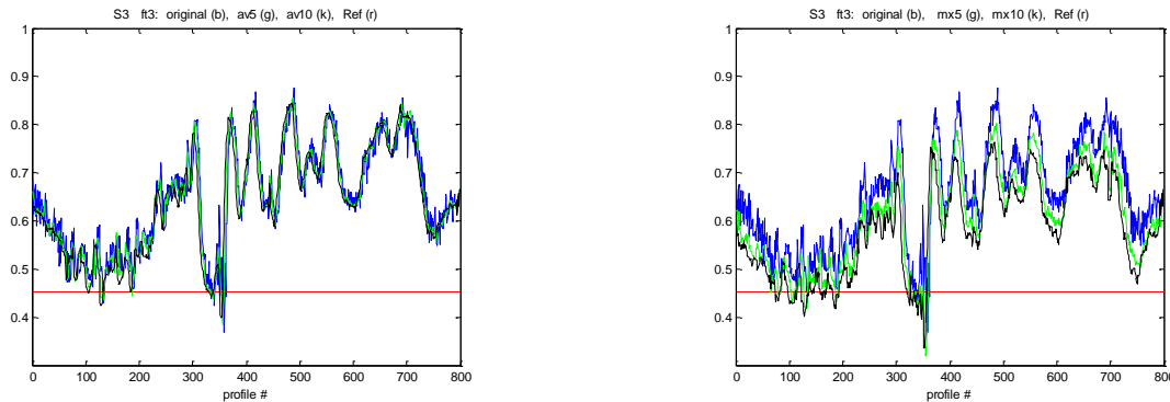
Figure 22: comparison of different ways to compute the test features (S3, ft3): averaging (left) or maxing (right) for L=1 (blue), L=5 (green), L=10 (black) (red line = overall reference).
